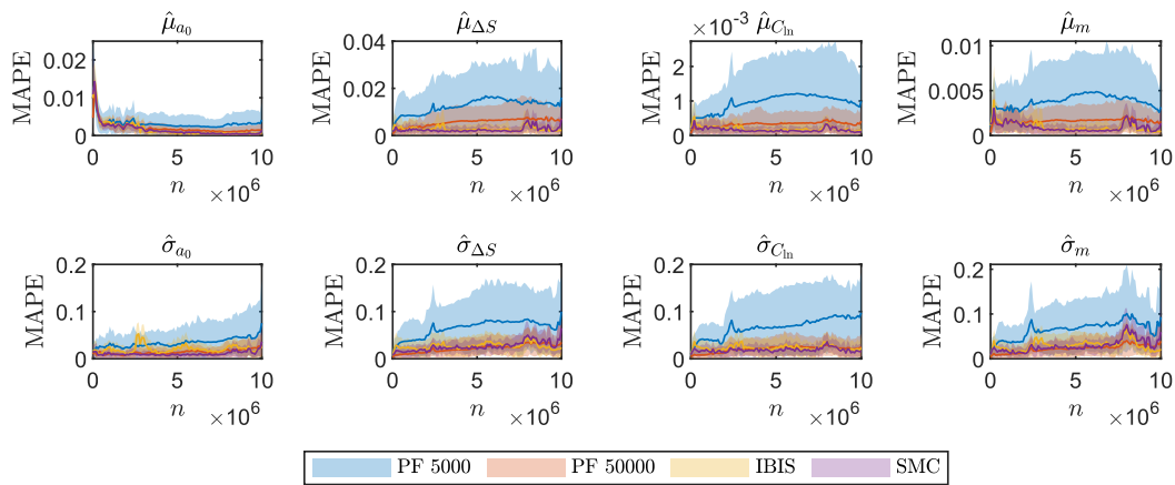
Figure 1: Comparison of the MAPE evaluated for the three different applied filters. The full lines show the mean and the shaded areas the 90% credible intervals from 50 different runs of the different algorithms.
